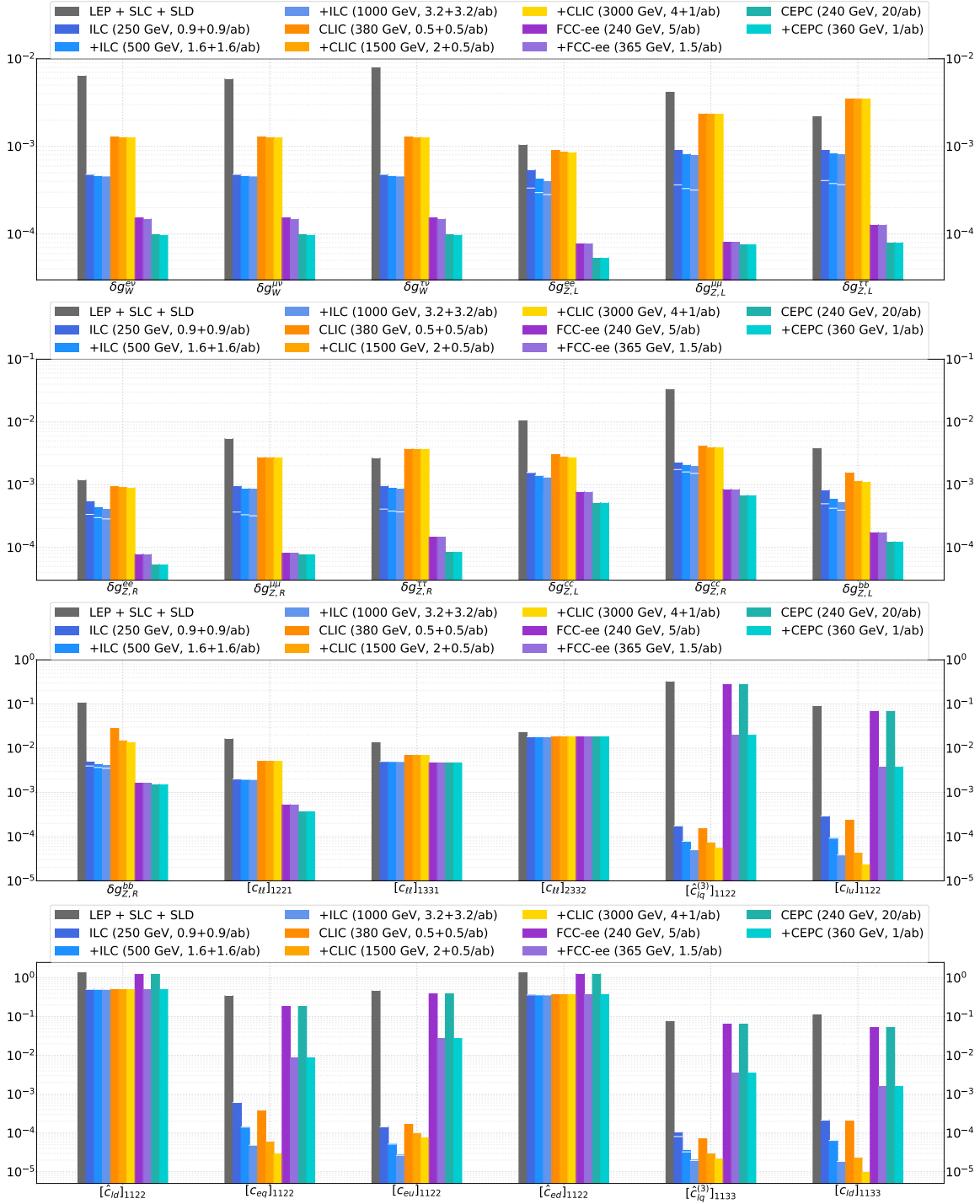
Figure 10: Precision reach on the 4-fermion operators and electroweak effective couplings from a SMEFT global fit at various future lepton colliders. "LEP+SLC+SLD" represents current measurements which are always combined in the future collider scenarios. The horizontal white line for ILC illustrates the global fit results when the pole observables from its Giga-Z option are included.
