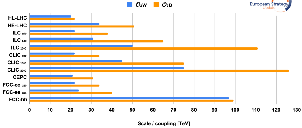
Figure 16: Exclusion reach of different colliders on four-fermion contact interactions from the operators O_{2W} and O_{2B} (figure taken from Ref. [158]).
